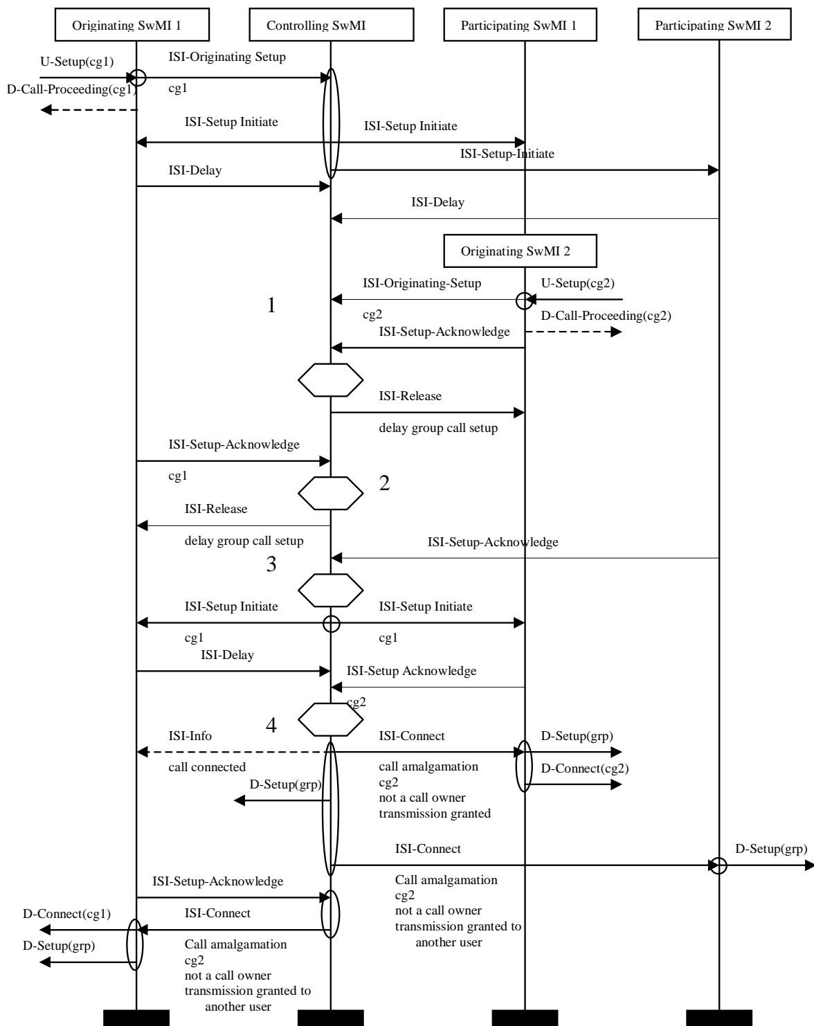
Figure E.7: Successful group call set-up: multiple calling parties the second calling OSwMI is ready first, the new setup from the second OSwMI is received while the CSwMI is activating the call
