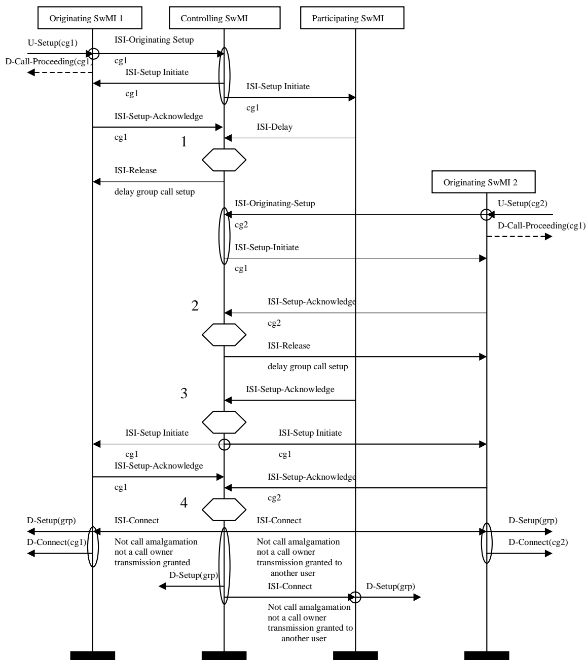
Figure E.8: Successful group call set-up: multiple calling parties the second calling OSwMI is ready first
