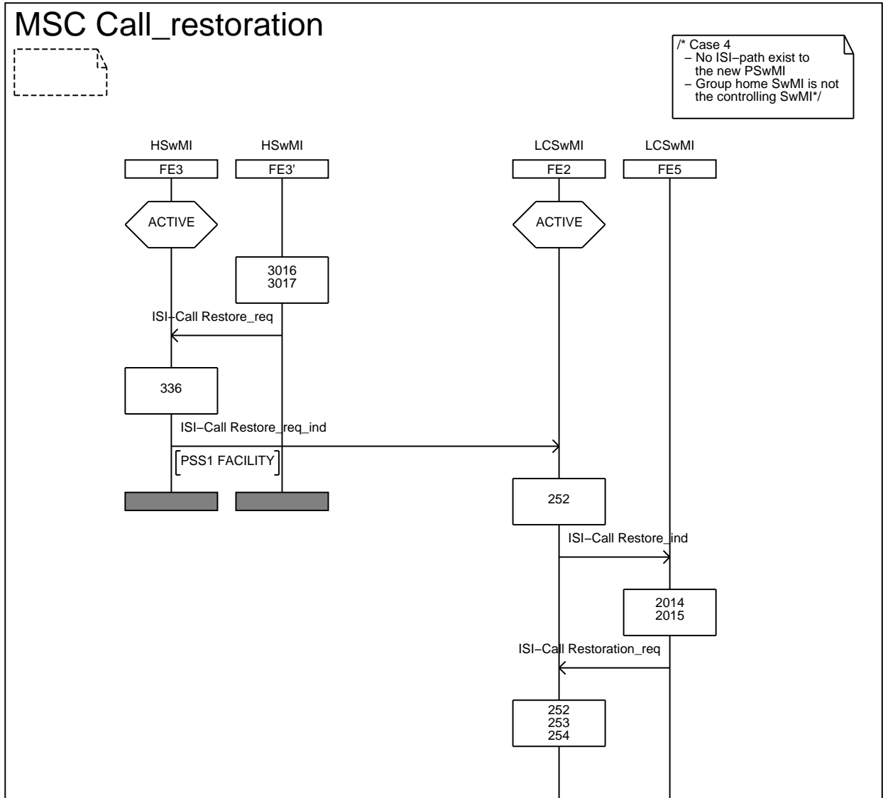
Figure 65: Information flow sequence - Group call restoration, case 4
