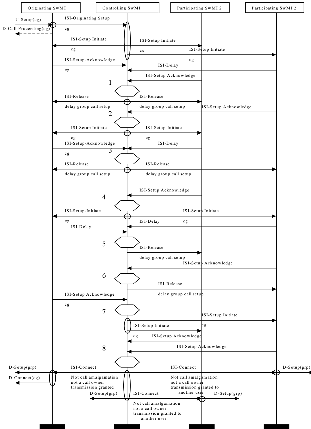
Figure E.4: Successful group call set-up: single calling party, some queuing for resources, showing multiple releasing
