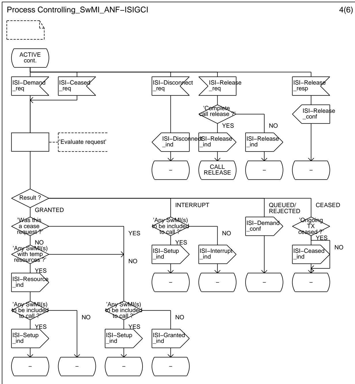
Figure A.8: SDL for group home/controlling SwMI ANF-ISIGC entity
