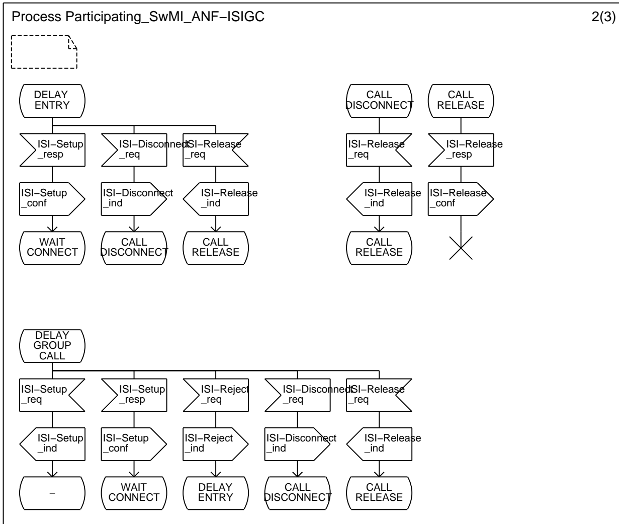
Figure A.10: SDL for participating SwMI ANF-ISIGC entity
