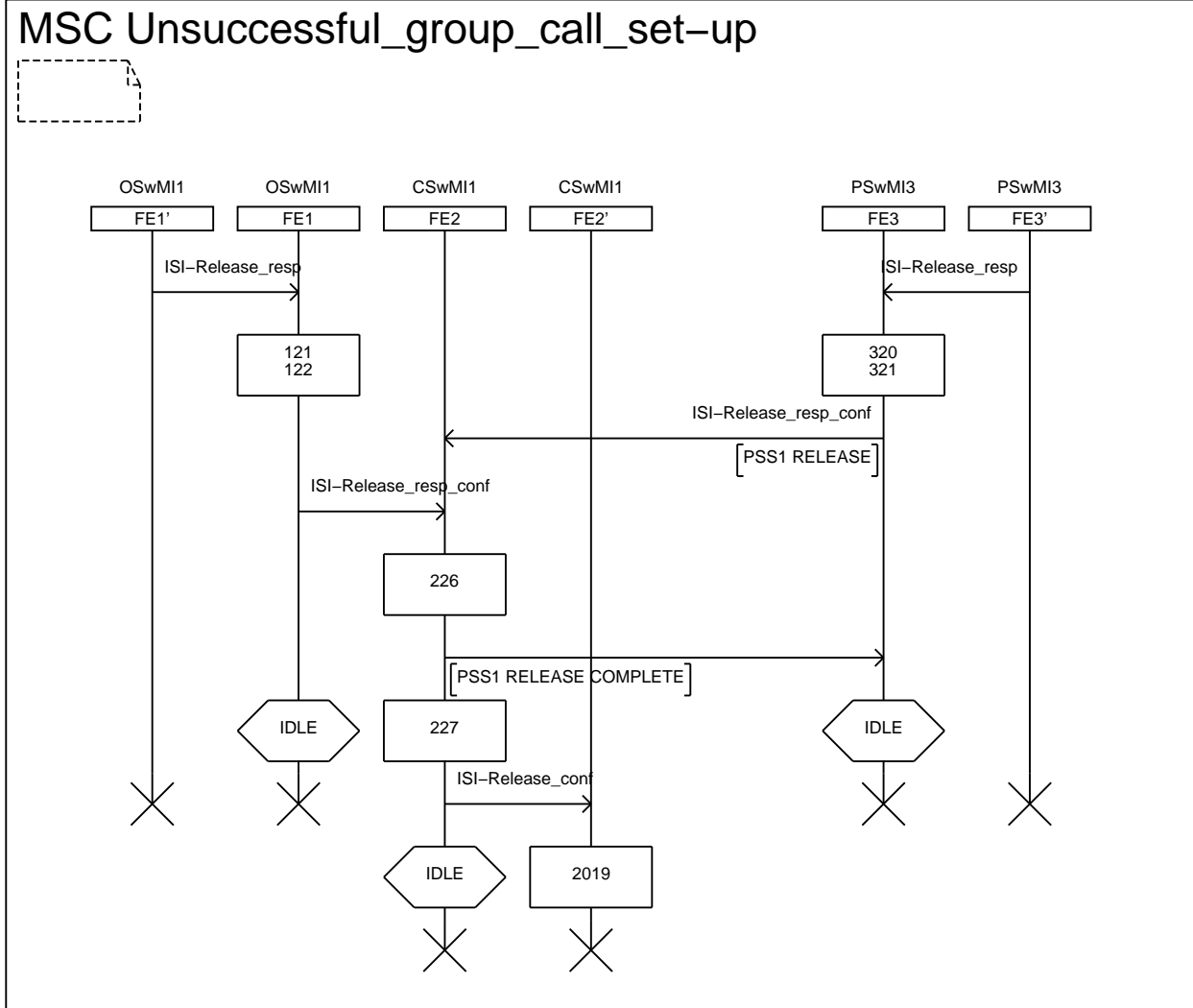
Figure 45: Information flow sequence - new B-channel not accepted (sheet 2 of 2)
