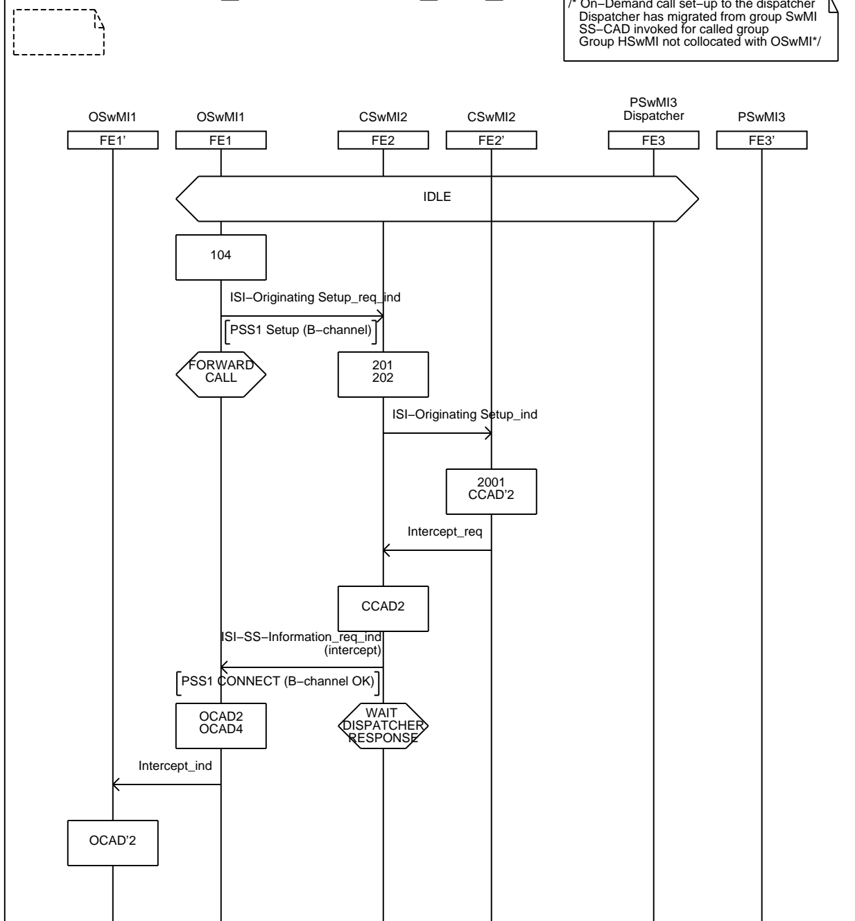
Figure B.9: Information flow sequence - On-demand call set-up (sheet 1 of 2)
