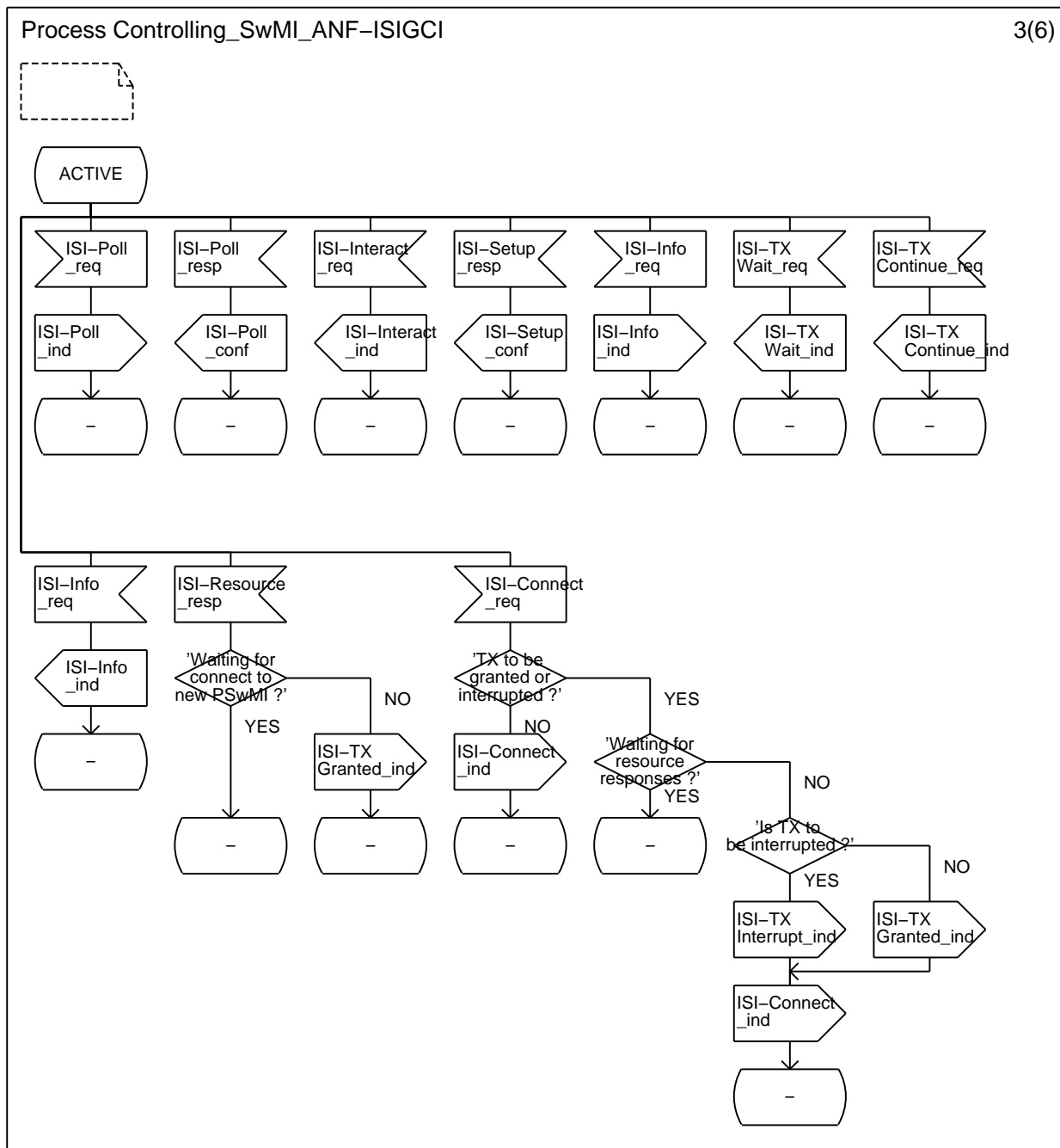
Figure A.7: SDL for group home/controlling SwMI ANF-ISIGC entity
