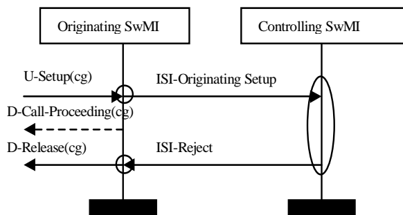
Figure E.23: Unsuccessful group call establishment, rejected by the CSwMI
