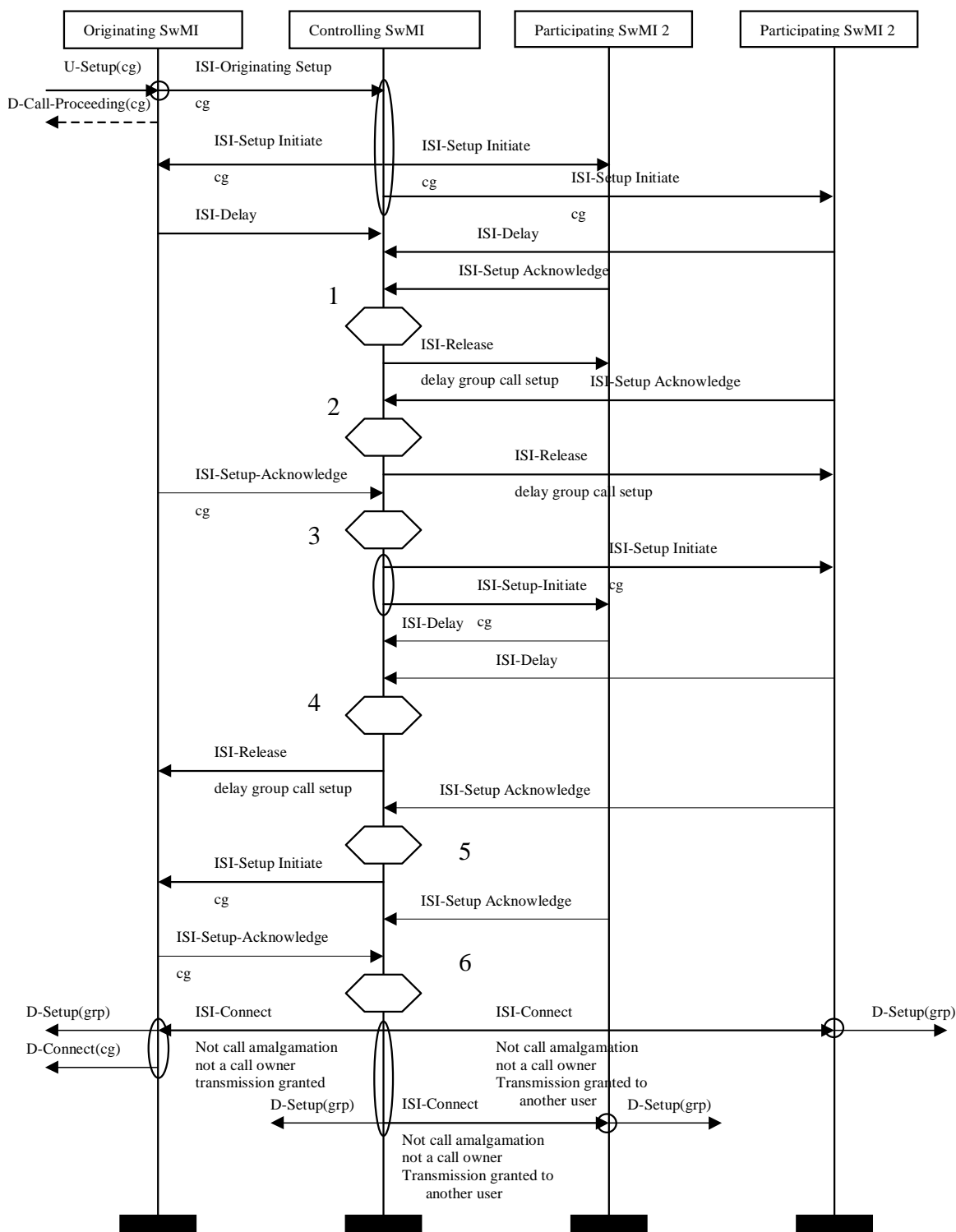
Figure E.3: Successful group call set-up: single calling party, some queuing for resources, different connect strategy to clause E.1.2
