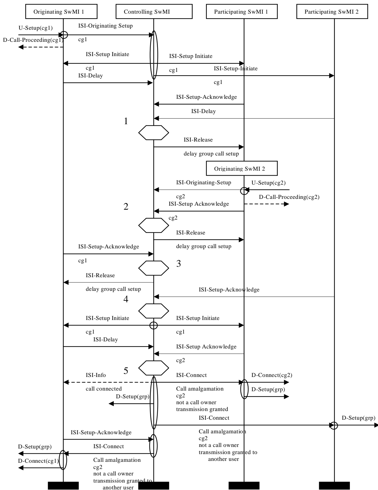
Figure E.6: Successful group call set-up: multiple calling parties the second calling OSwMI is ready first, the new setup from the second OSwMI is received while the CSwMI is delaying the call
