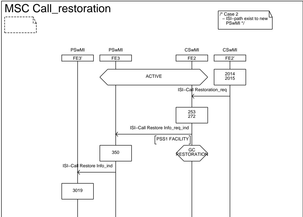
Figure 63: Information flow sequence - Group call restoration, case 2 (sheet 2 of 2)
