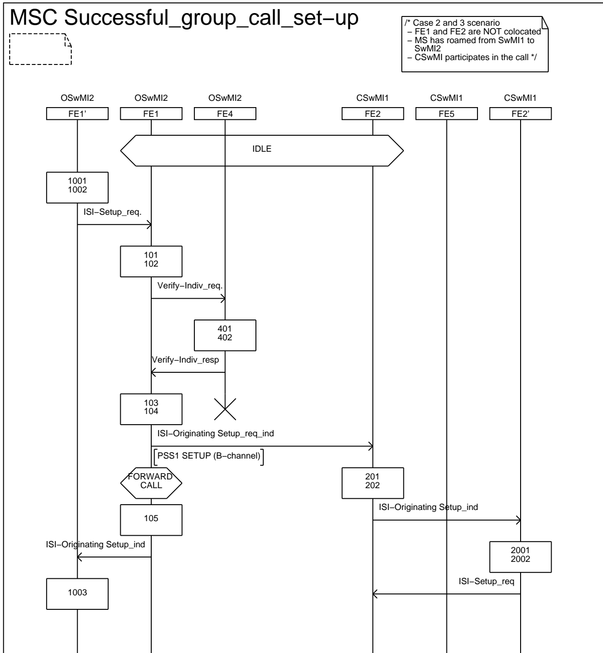
Figure 23: Information flow sequence - successful group call set-up, case 2 and 3 (sheet 1 of 4)
