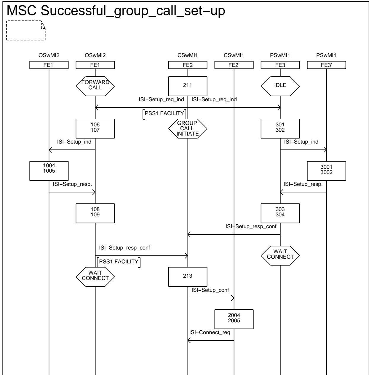
Figure 25: Information flow sequence - successful group call set-up, case 2 and 3 (sheet 3 of 4)
