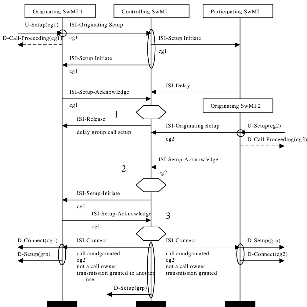
Figure E.12: Successful group call set-up: multiple calling parties and no PSwMI
